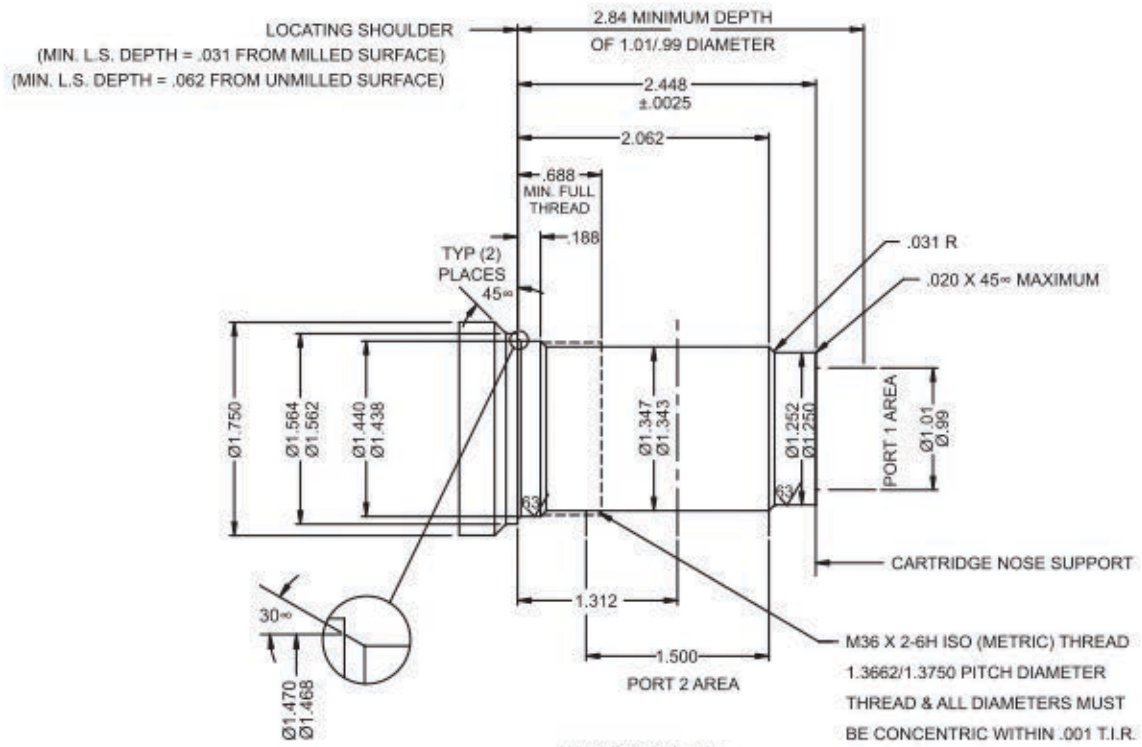
T-16A Cavity
